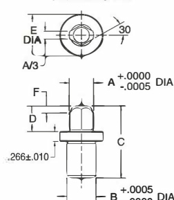
Press-Fit Type Diamond Pin
