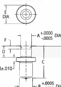
Press-Fit Type Round Pin
